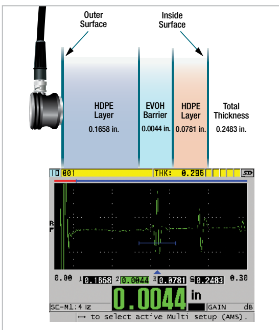
The 38DL PLUS thickness gauge can make accurate measurements of up to four individual layers simultaneously.
