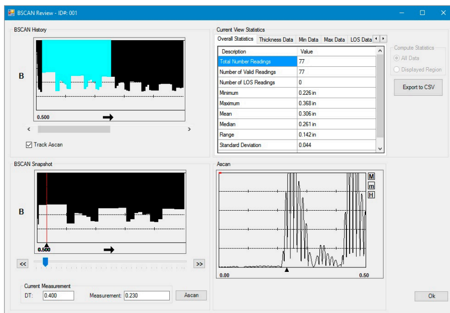
B-scan review in the GageView Thickness program
