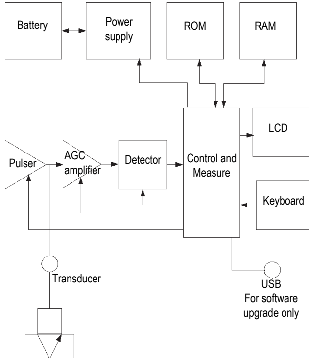
Figure 9-1 27MG block diagram
