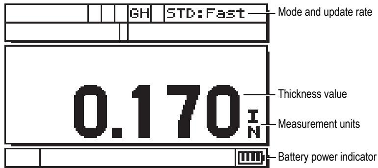
Figure 3-1 The measurement screen
