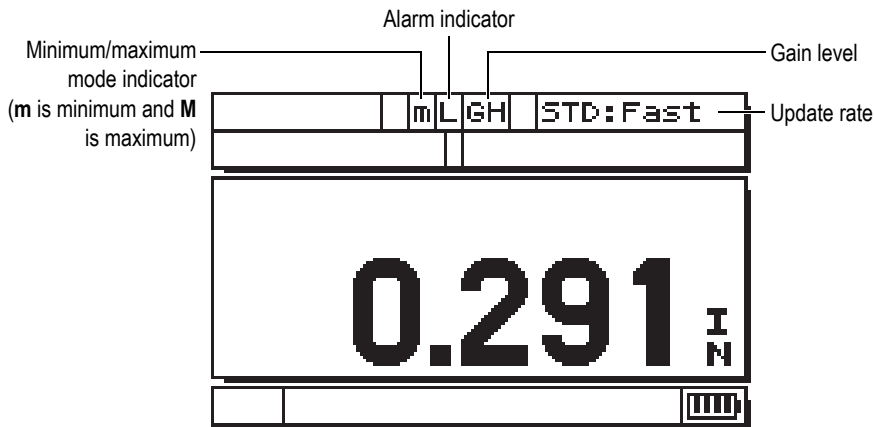
Figure 3-2 Other elements of the measurement screen
