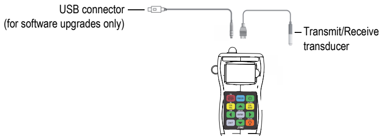
Figure 1-2 The 27MG connections
