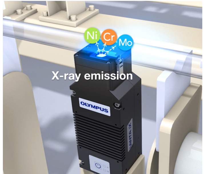
Example of the Vanta iX material verification system testing a fabricated metal pipe on a cross transfer table.
