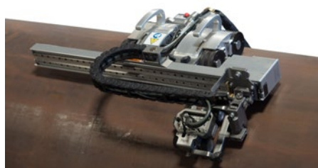
The SteerROVER scanner, when fitted with a motorized raster arm, is a powerful solution for corrosion inspection in remote locations.
